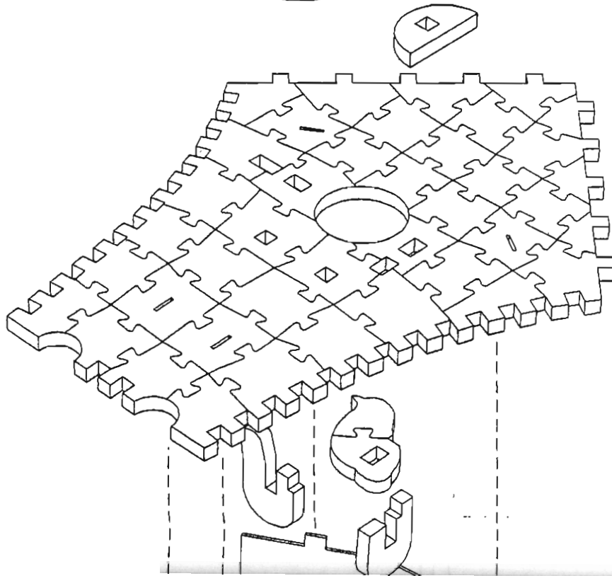
Front Assembly
