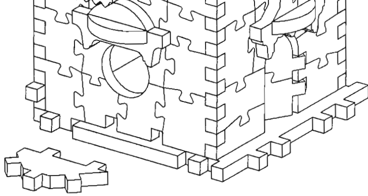
Assembly 3
