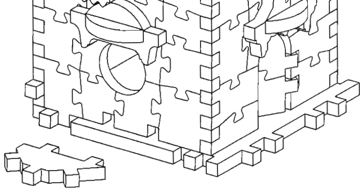
Assembly 3
