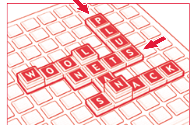
Figure 7 Score: 16 Points
