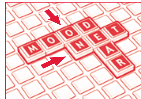
Figure 3 Score: 10 Points
